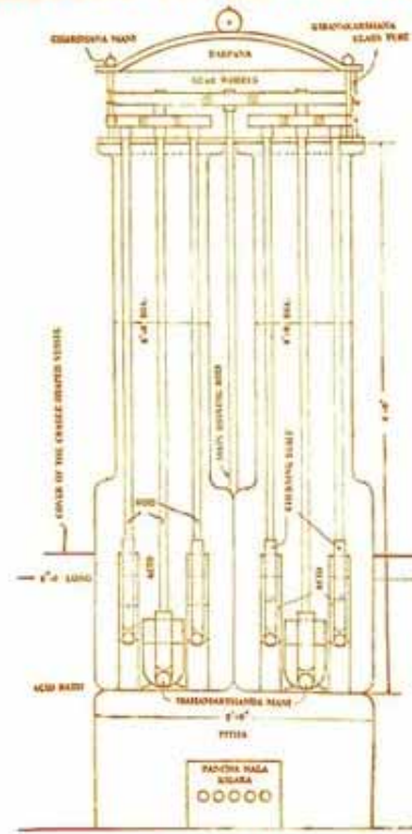
SECTIONAL ELEVATION
